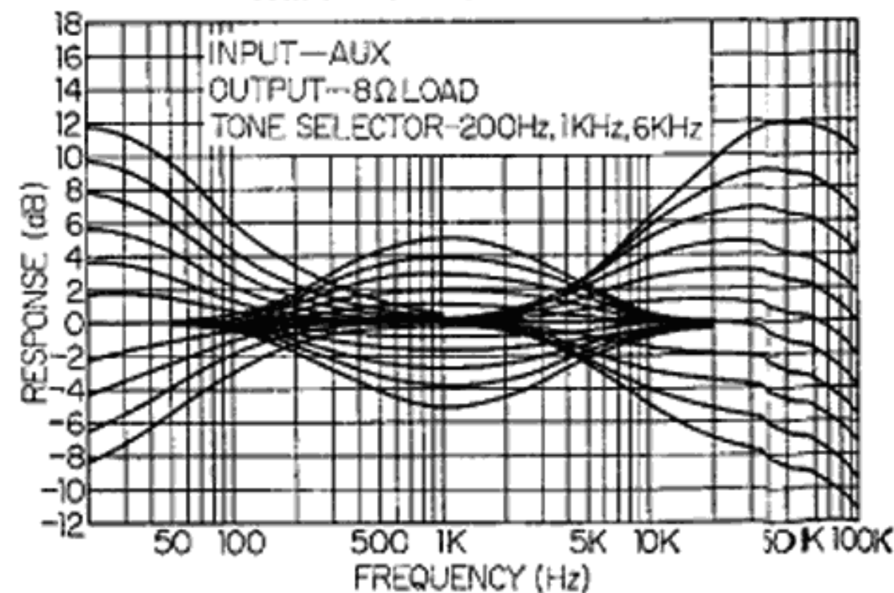
TRIPLETONE CONTROL
