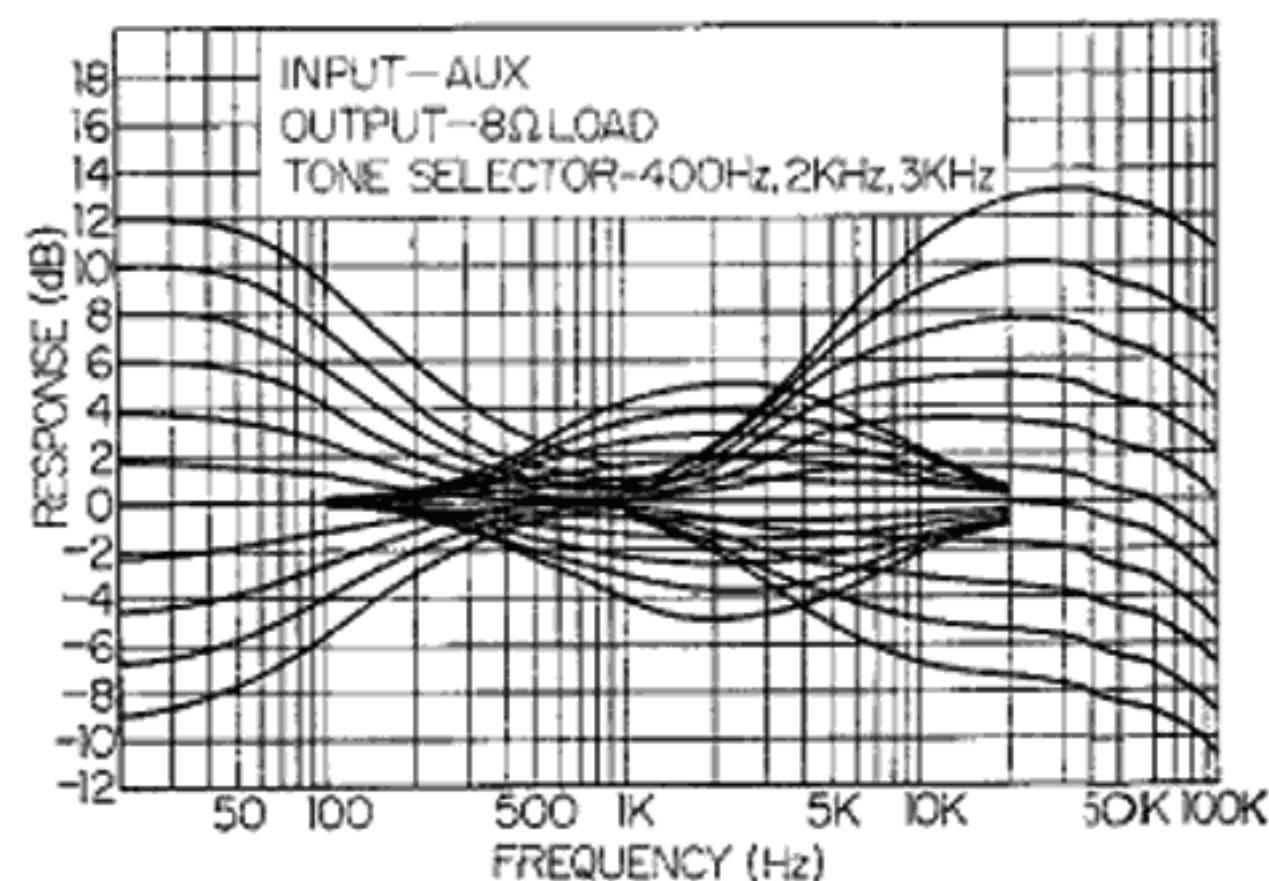
TRIPLETONE CONTROL
