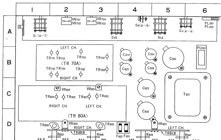
TOP VIEW OF UPPER CHASSIS
